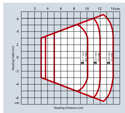
PDF417 reading zone
