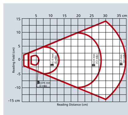
Standard reading zone
